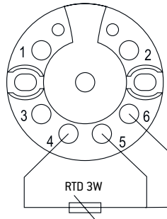
RESISTANCE THERMOMETER
